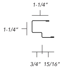
Wall Channel with reveal (painted one side only) (Aluminum) 252575 60.00.415
