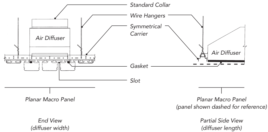
Air Diffuser Unit - Section Details (2 Slot, 8" Collar, 9" Width)
