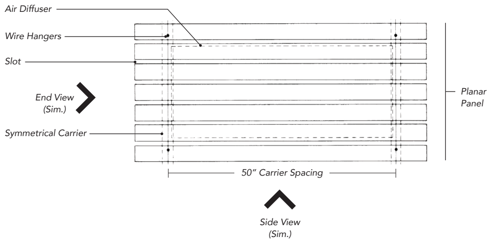
Air Diffuser Unit - Plan Detail (4 Slot, 10" Collar, 17" Width)
