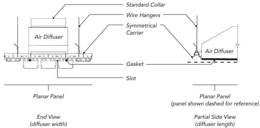
Air Diffuser Unit - Section Detail (2 Slot, 8" Collar, 9" Width)
