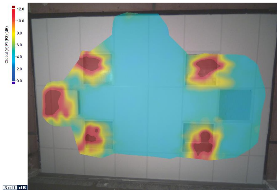
Fig. 7 - A color map showing sound being absorbed by a stone wool panel acoustic ceiling with a NRC rating of 0.95 (blue).
